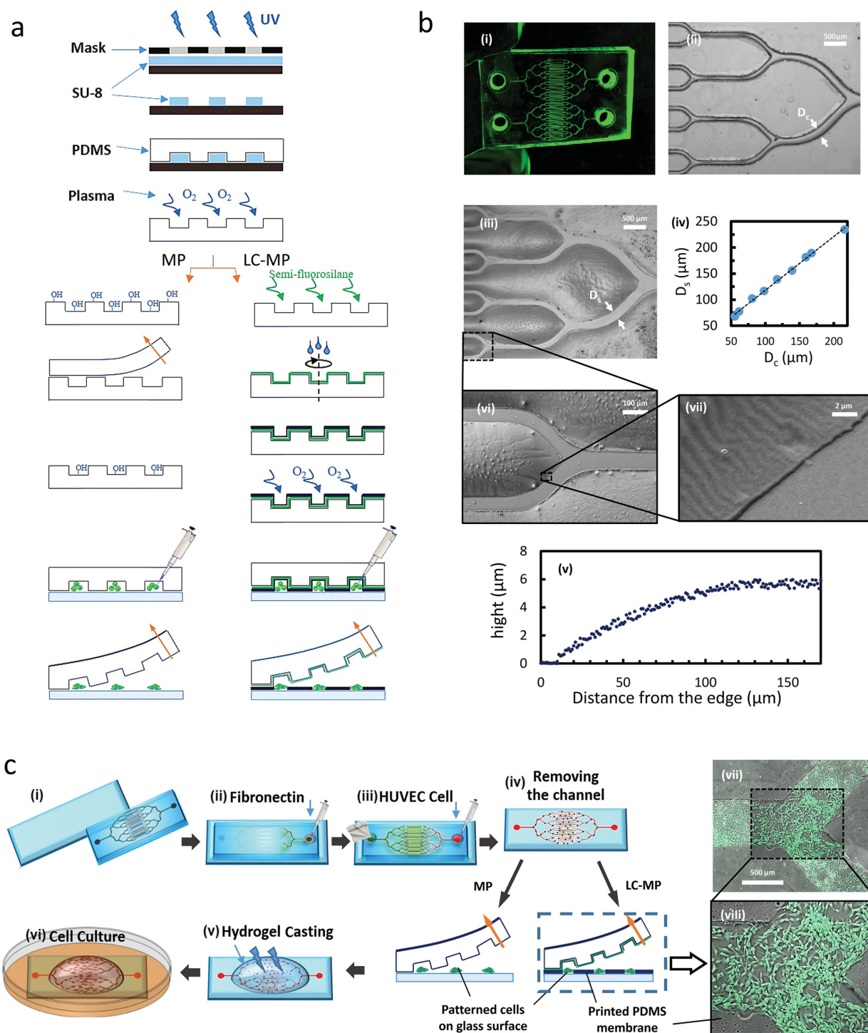
Figure 1. Demonstration of laterally confined microfluidic patterning method used for cell and protein patterning, and hydrogels. a) Schematic of the fabrication procedure followed to make MP and LC-MP devices. b) (i) Microfluidic PDMS channel device with (ii) detailed dimension of the channels ( D_c is defined as the width of the PDMS channels). (iii) PDMS membrane printed on glass surface ( D_s is defined as the width of the printed microstructure created on the surface). (iv) The width of the printed membrane pattern on the surface ( D_s ) versus the width of its corresponding PDMS channel ( D_c ) is depicted. (v) The profile of membrane was measured with respect to the edge of membrane using a profilometer (height = 0 is the glass surface). (vi) Magnified image of a printed junction on a glass substrate. (vii) SEM image of the patterned PDMS membrane on a glass, showing the thickness of the PDMS membrane at the edge is less than a micron. c) Initially, (i) the glass substrate and the microfluidics channels are oxygen plasma treated. (ii) Microfluidic PDMS channels are assembled on the glass substrate and fibronectin solution is loaded into the inlet port. (iii) After 1 h incubation, the solution is collected from the outlet and meanwhile the solution containing HUVECs is loaded in the inlet (forced capillary). (iv) After 1 h incubation, the PDMS channel is removed and cultured for 1 d before casting the hydrogel. (v) Hydrogel is casted on the sample. (vi) The glass substrate is then immersed in the cell media and cultured. (vii) Patterned HUVECs on the glass surface (using LC-MP method) with PDMS membrane confining the cells. (viii) Magnified image of the patterned cells and the PDMS membrane.
